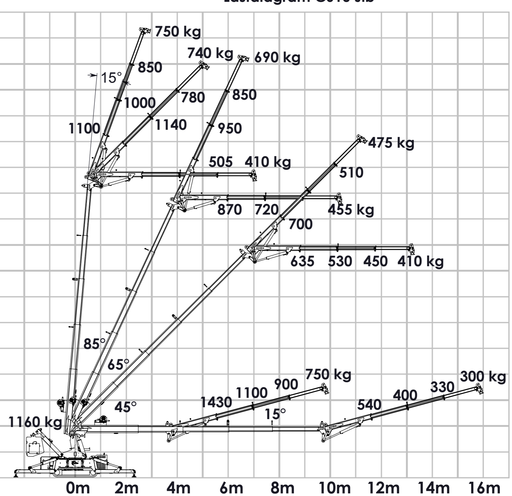
Lastdiagram C610 Jib
